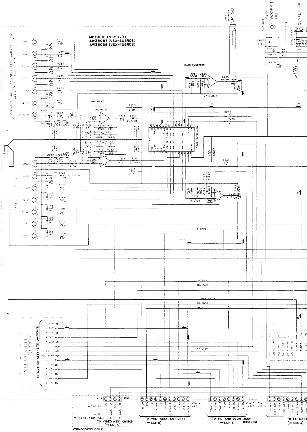
MOTHER ASSY (1/3)
