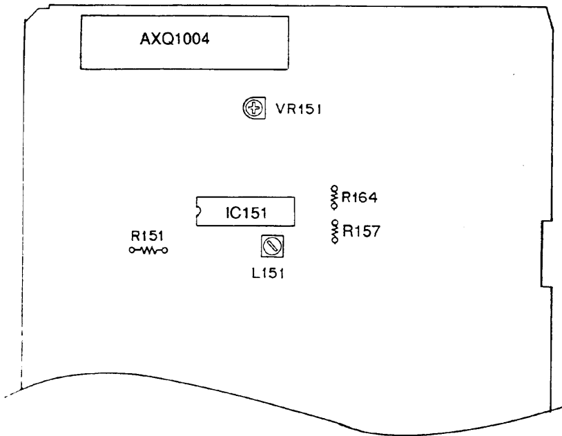
Fig. 1-2. Adjustment Points
