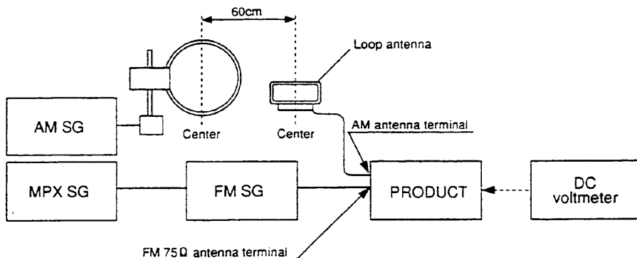
Fig. 1-1. AM and FM Adjustment Wiring Diagram
