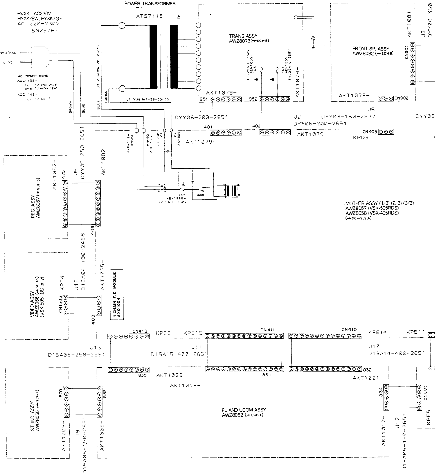
OVERALL SCHEMATIC DIAGRAM
